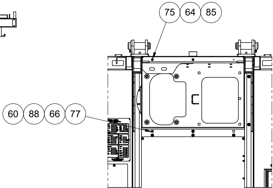
SECTION F-F
