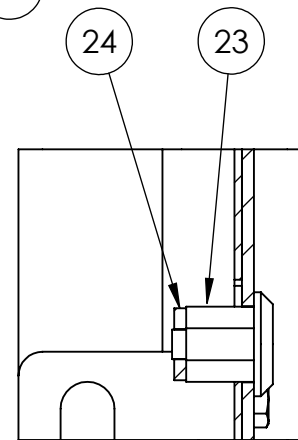
DETAIL F-F
